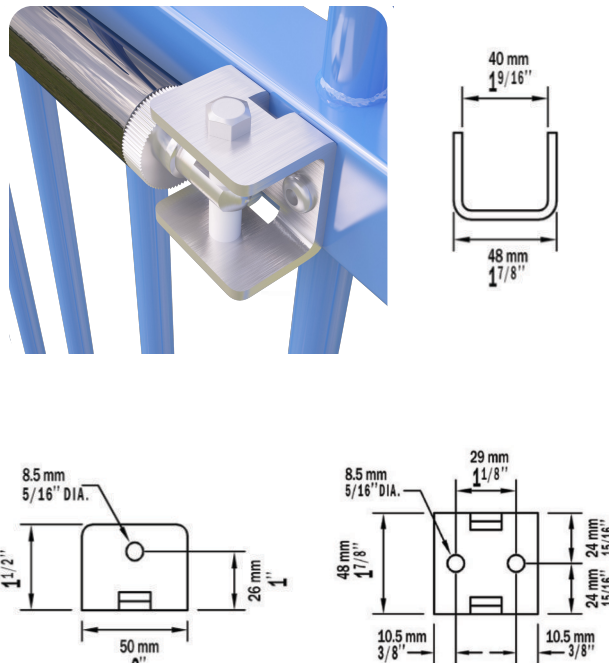
Gate Bracket
