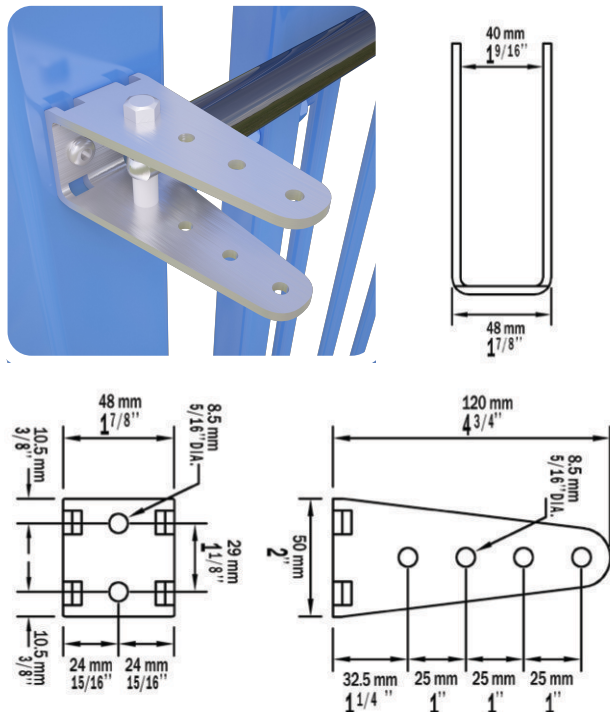
Post Bracket
